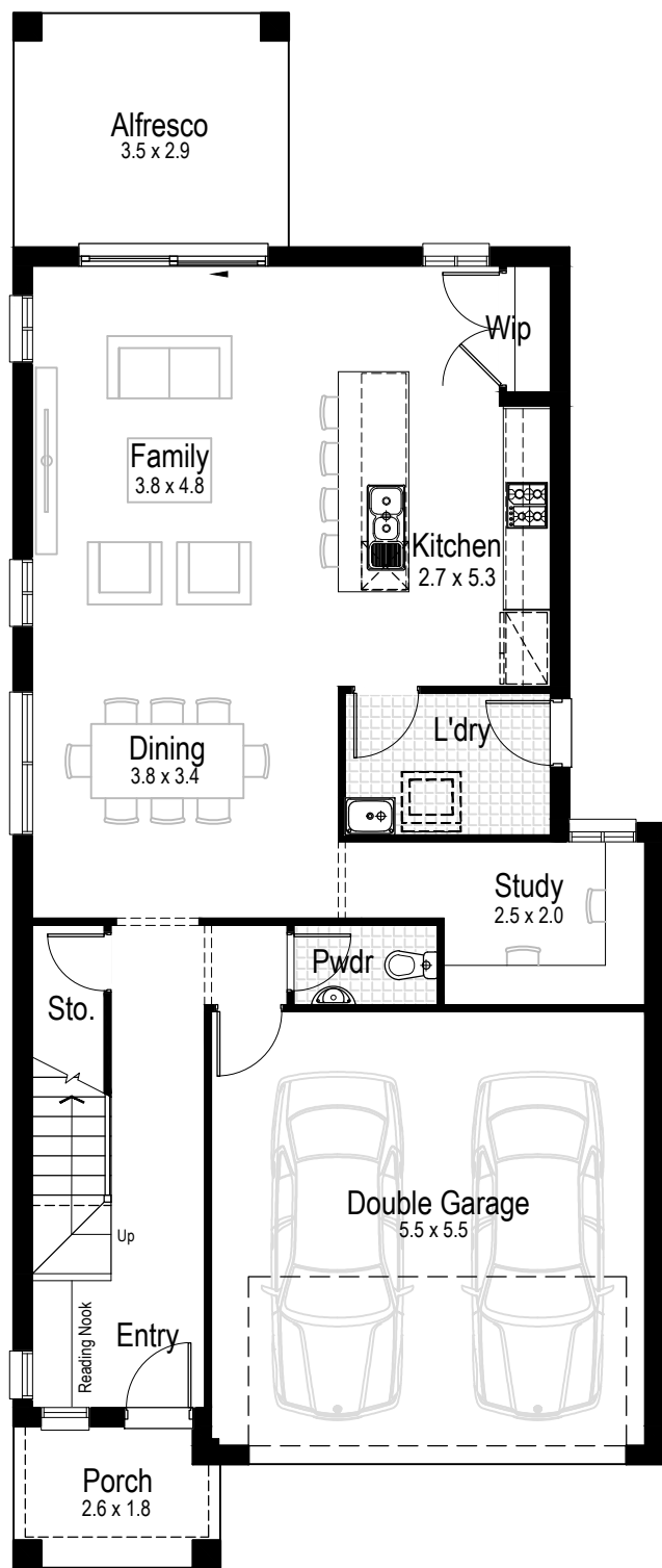
Ground Floor
